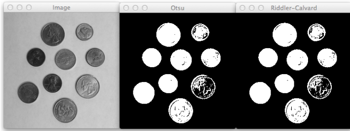
Figure 9.3: Left: The original grayscale coins image. Middle: Applying Otsu's method to find an optimal value of T . Right: Applying the Riddler-Calvard method to find an optimal value of T .
